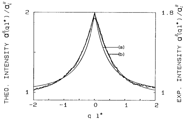
Fig. 5. — Experimental coherent backscattering peak for 0.46 \mu\text{m} polystyrene spheres (solid fraction 10 %) as a function of ql^* ( l^* = 20 \mu\text{m} ). (a) and (b) are theoretical predictions (see text).
