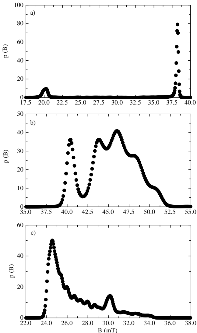
FIG. 2. a) The local field distribution in the intermediate state. A background of muons stopping in the cryostat shows an applied field of 20 mT, while the muons in the sample precess at a frequency corresponding to 38 mT. This corresponds to the critical field B_c at the temperature of 5.3 K, where the measurement was carried out. b) The local field distribution in the intermediate mixed state. The applied field can be seen to be 40 mT. In addition, there is a wide distribution of local fields corresponding to a vortex lattice at higher fields. The mean field of this flux lattice corresponds to the critical field at the transition from type-I to type-II behaviour T^{I-II} , if the overall field expulsion is taken into account (see text). The measurement was carried out at a temperature of 4.3 K. c) The field distribution for a vortex lattice, in the mixed state. The field distribution has a very characteristic shape, with a tail extending to fields higher than the average. The measurement was taken in an applied field of 30 mT in the type-II sample containing 5 % Bi.
